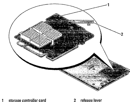
Figure 4-4. Removing and Installing the Storage Controller Card
