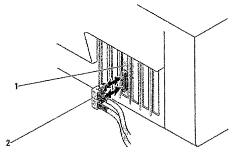
Figure 4-3. Connecting the Cable for 6Gbps SAS HBA
