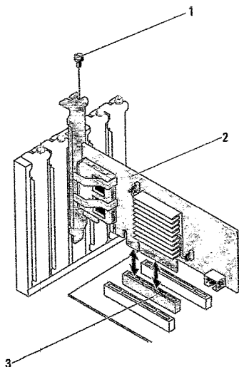
Figure 4-1. Installing a 6Gbps SAS HBA
